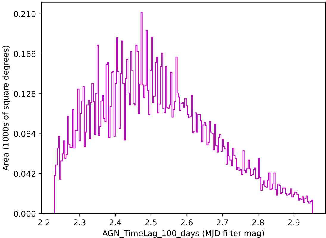
weather_cloudso35v3.4_10yrs z band: AGN_TimeLag_100_days
