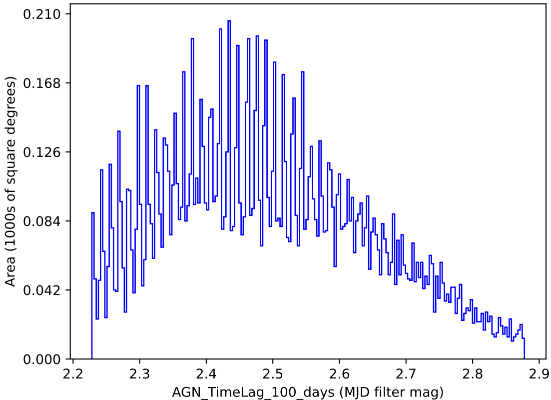
weather_cloudso35v3.4_10yrs y band: AGN_TimeLag_100_days
