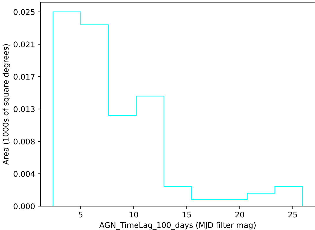
weather_cloudso35v3.4_10yrs u band: AGN_TimeLag_100_days
