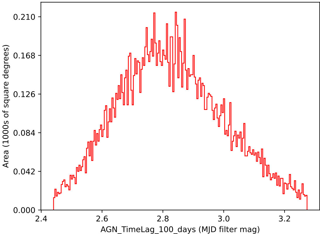
weather_cloudso35v3.4_10yrs i band: AGN_TimeLag_100_days
