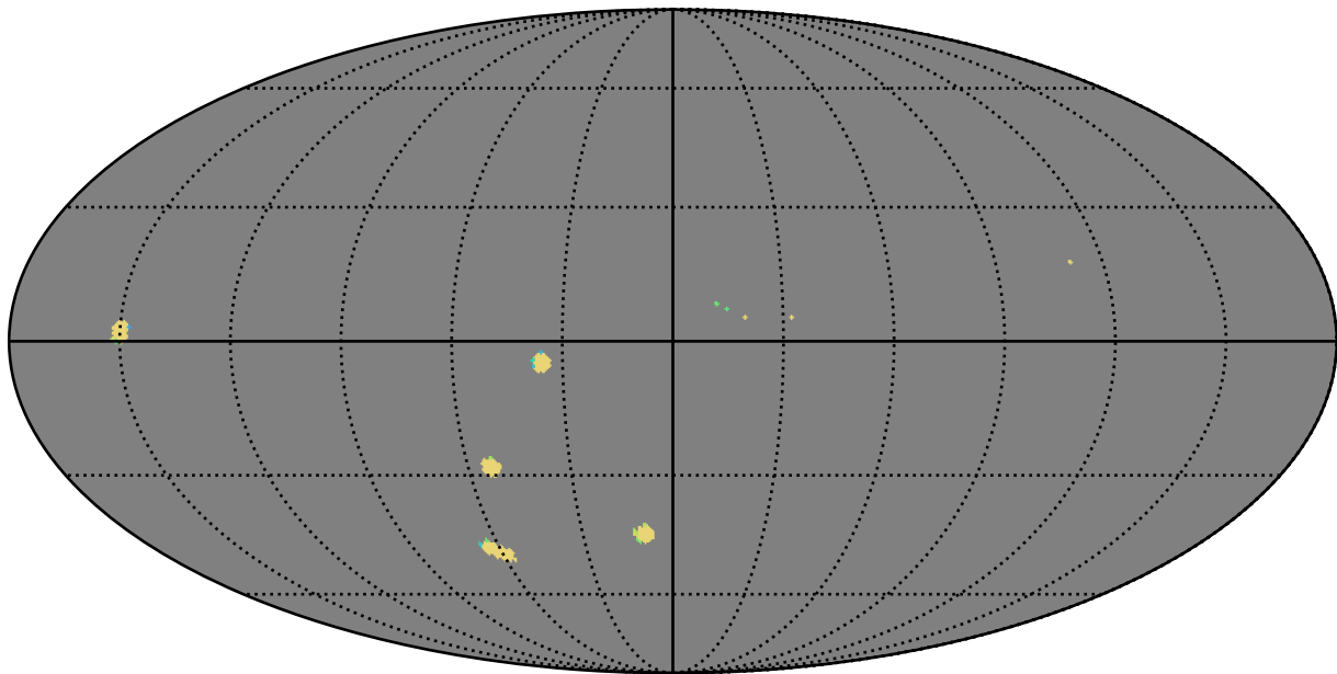
weather_cloudso35v3.4_10yrs g band: AGN_TimeLag_100_days
