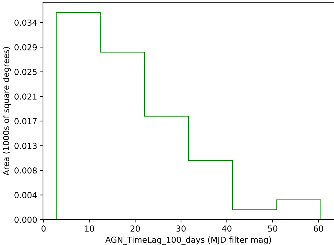
weather_cloudso35v3.4_10yrs g band: AGN_TimeLag_100_days
