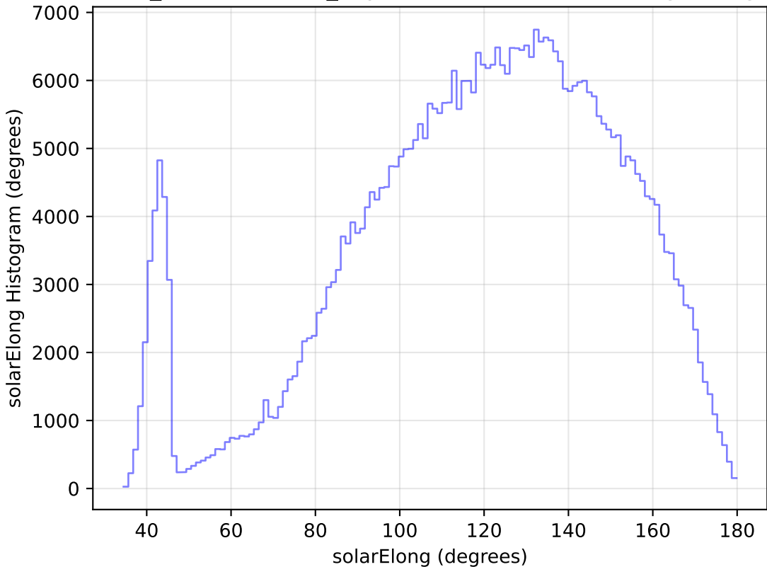
weather_cloudso35v3.4_10yrs WFD z band: solarElong Histogram
