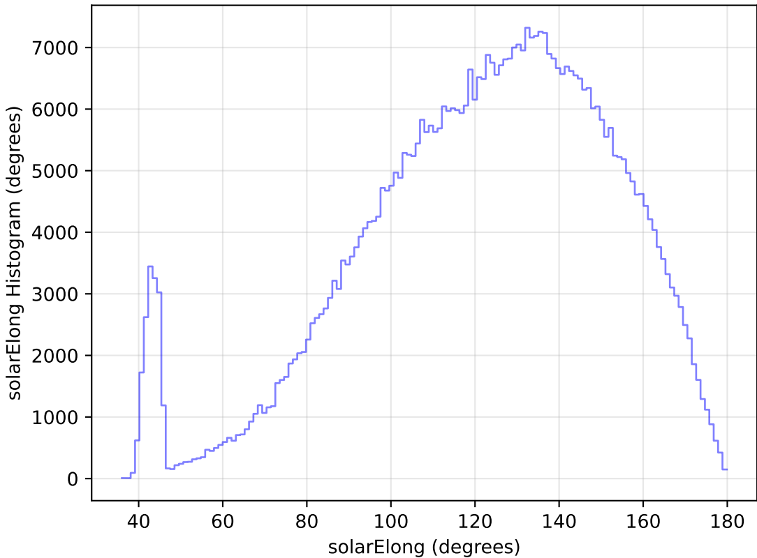
weather_cloudso35v3.4_10yrs WFD r band: solarElong Histogram
