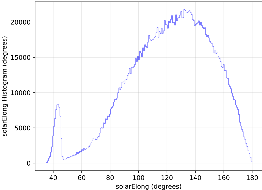
weather_cloudso35v3.4_10yrs WFD all bands: solarElong Histogram
