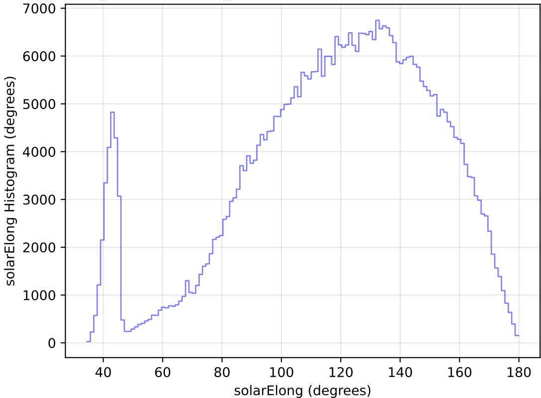
weather_cloudso35v3.4_10yrs All sky z band: solarElong Histogram
