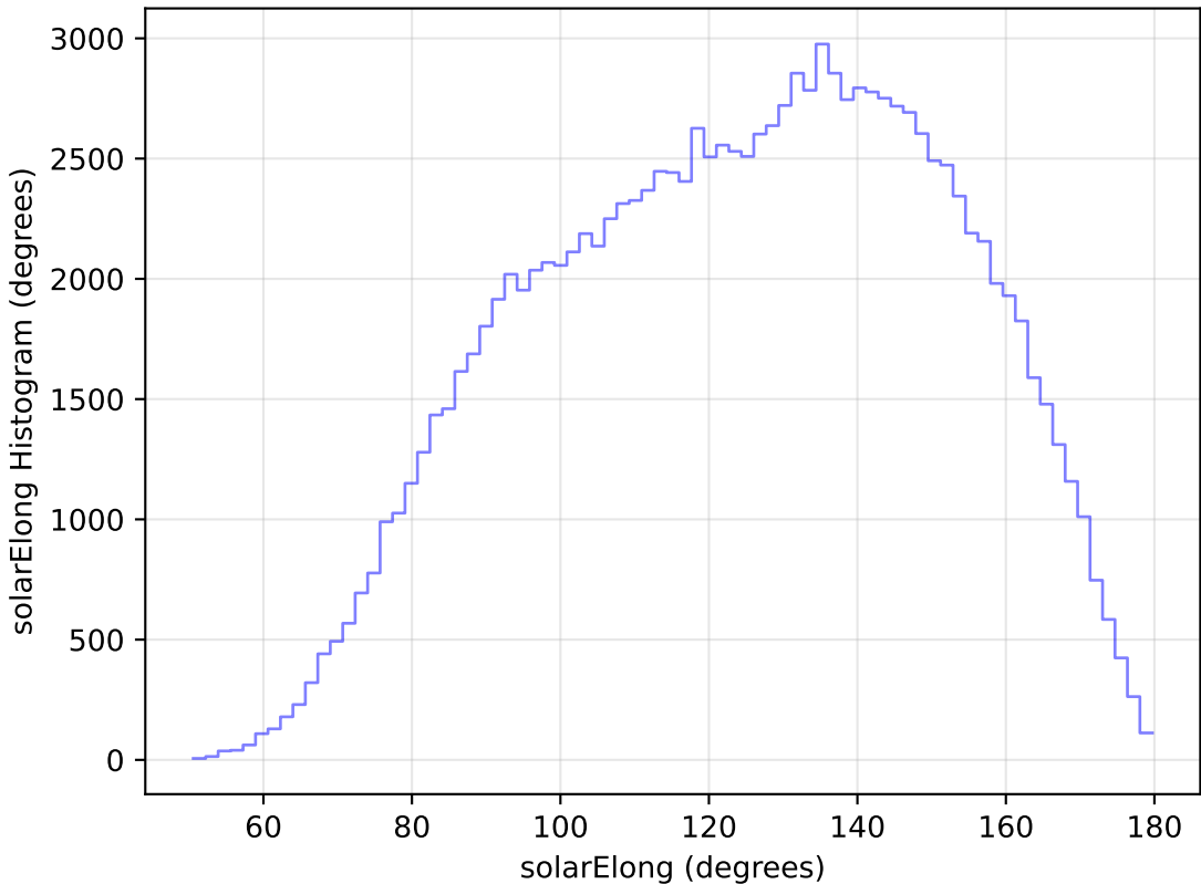
weather_cloudso35v3.4_10yrs All sky u band: solarElong Histogram
