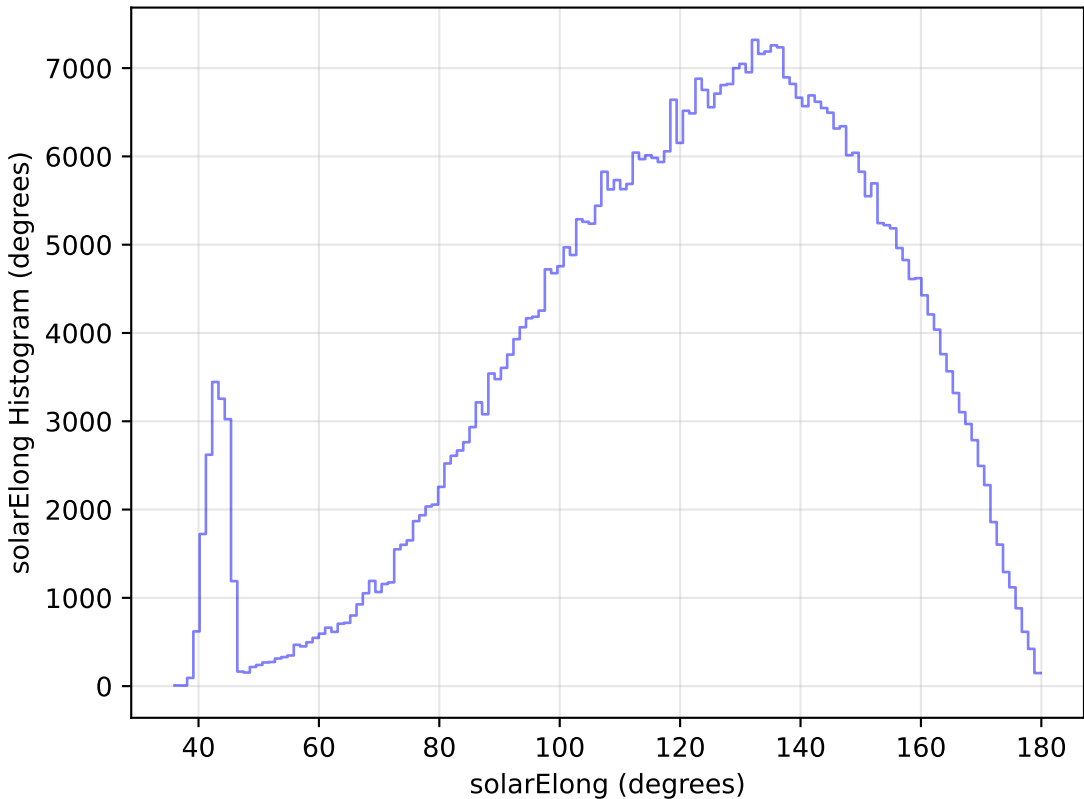
weather_cloudso35v3.4_10yrs All sky r band: solarElong Histogram
