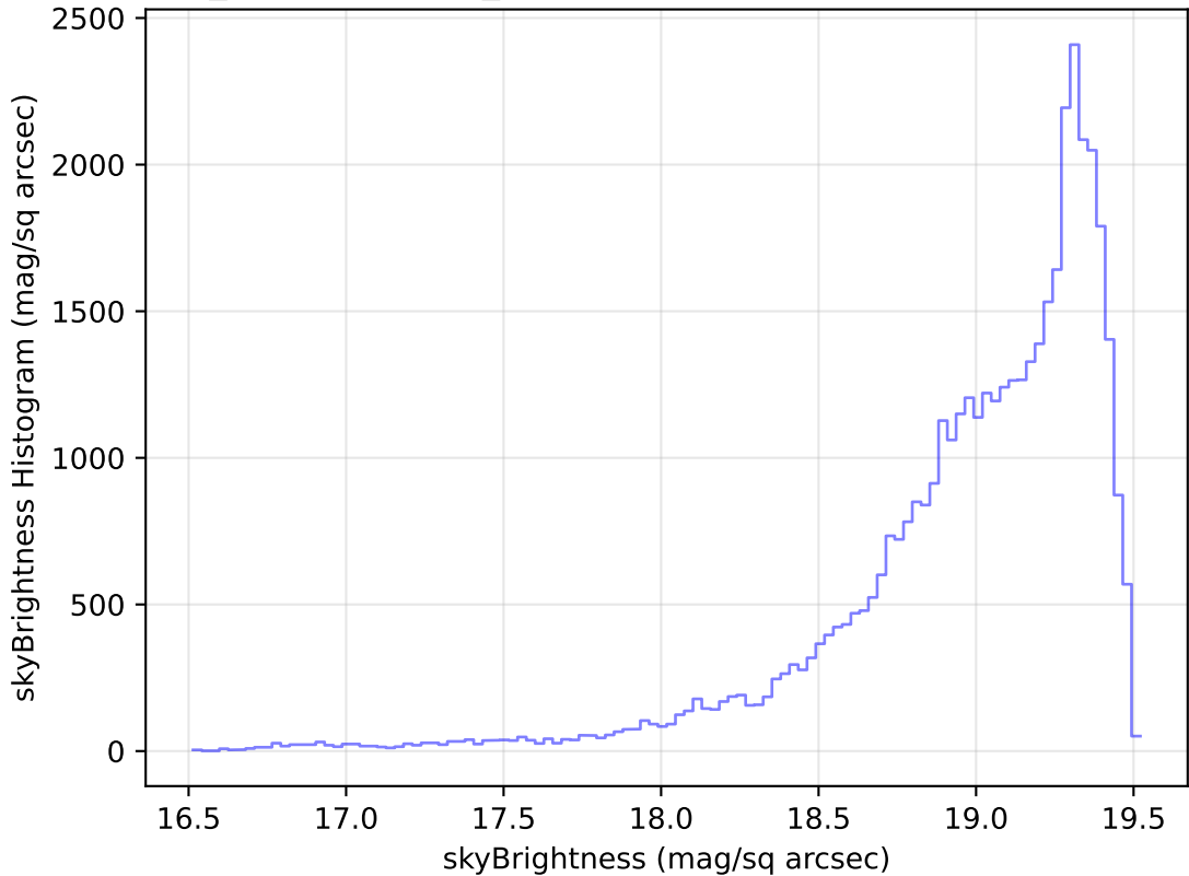
weather_cloudso35v3.4_10yrs Yr 1 z band: skyBrightness Histogram
