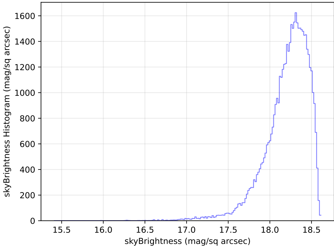
weather_cloudso35v3.4_10yrs Yr 1 y band: skyBrightness Histogram
