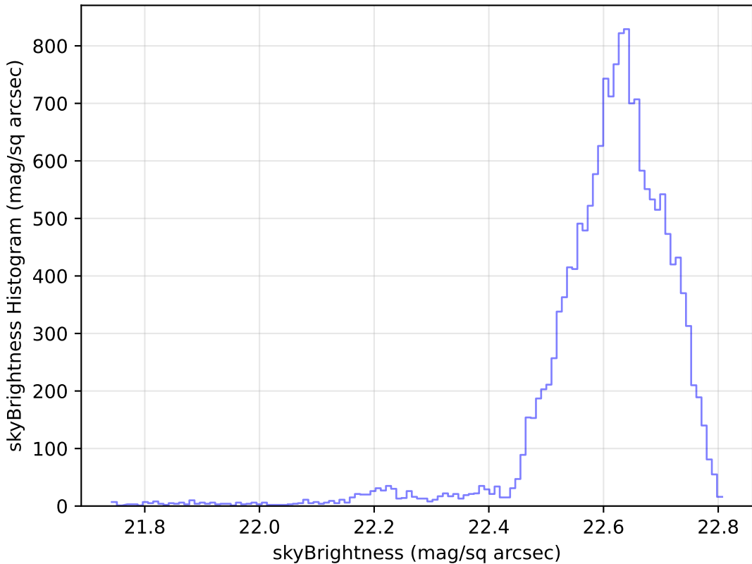
weather_cloudso35v3.4_10yrs Yr 1 u band: skyBrightness Histogram
