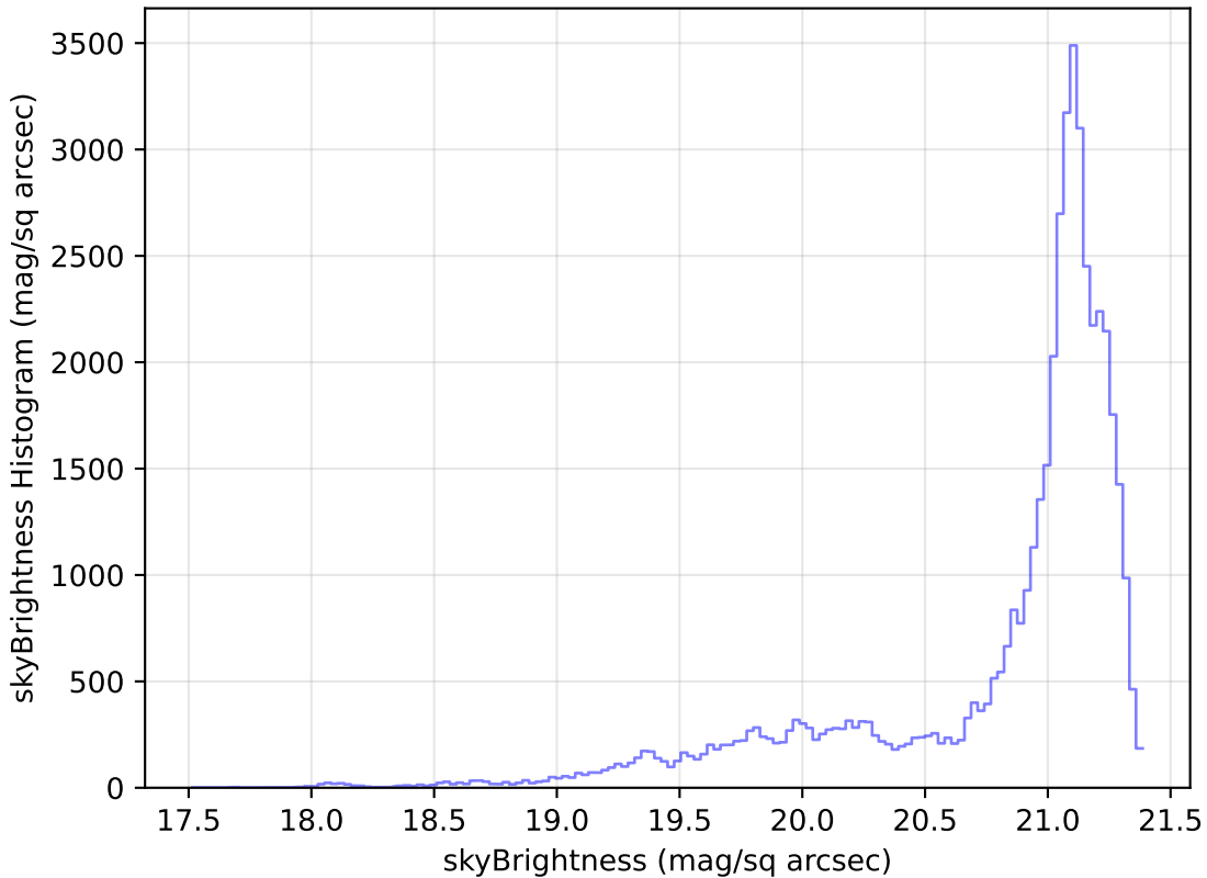
weather_cloudso35v3.4_10yrs Yr 1 r band: skyBrightness Histogram
