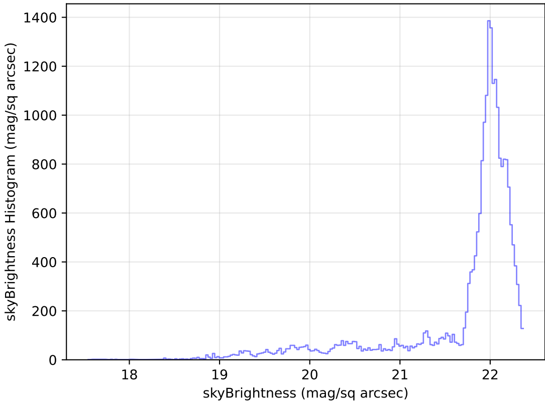
weather_cloudso35v3.4_10yrs Yr 1 g band: skyBrightness Histogram
