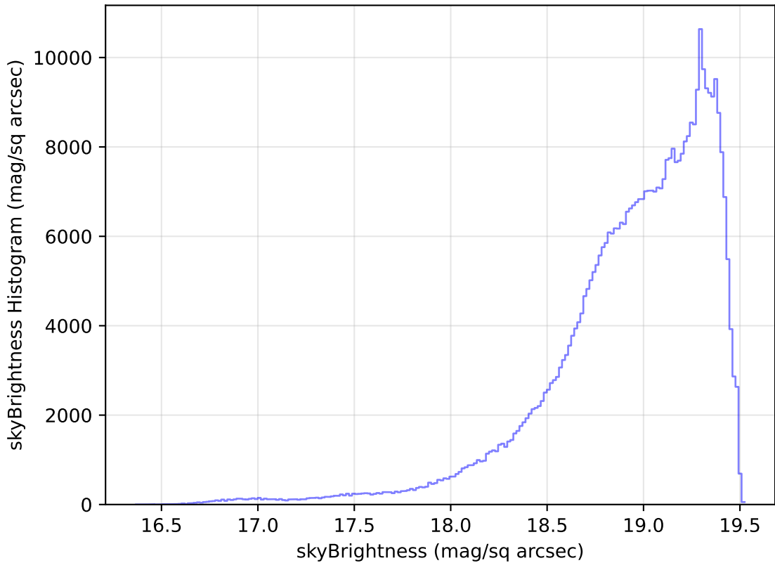
weather_cloudso35v3.4_10yrs WFD z band: skyBrightness Histogram
