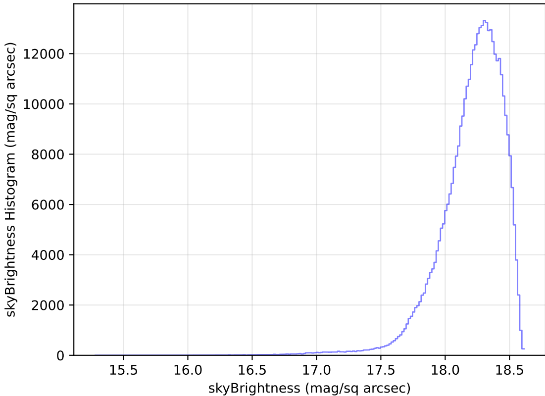
weather_cloudso35v3.4_10yrs WFD y band: skyBrightness Histogram
