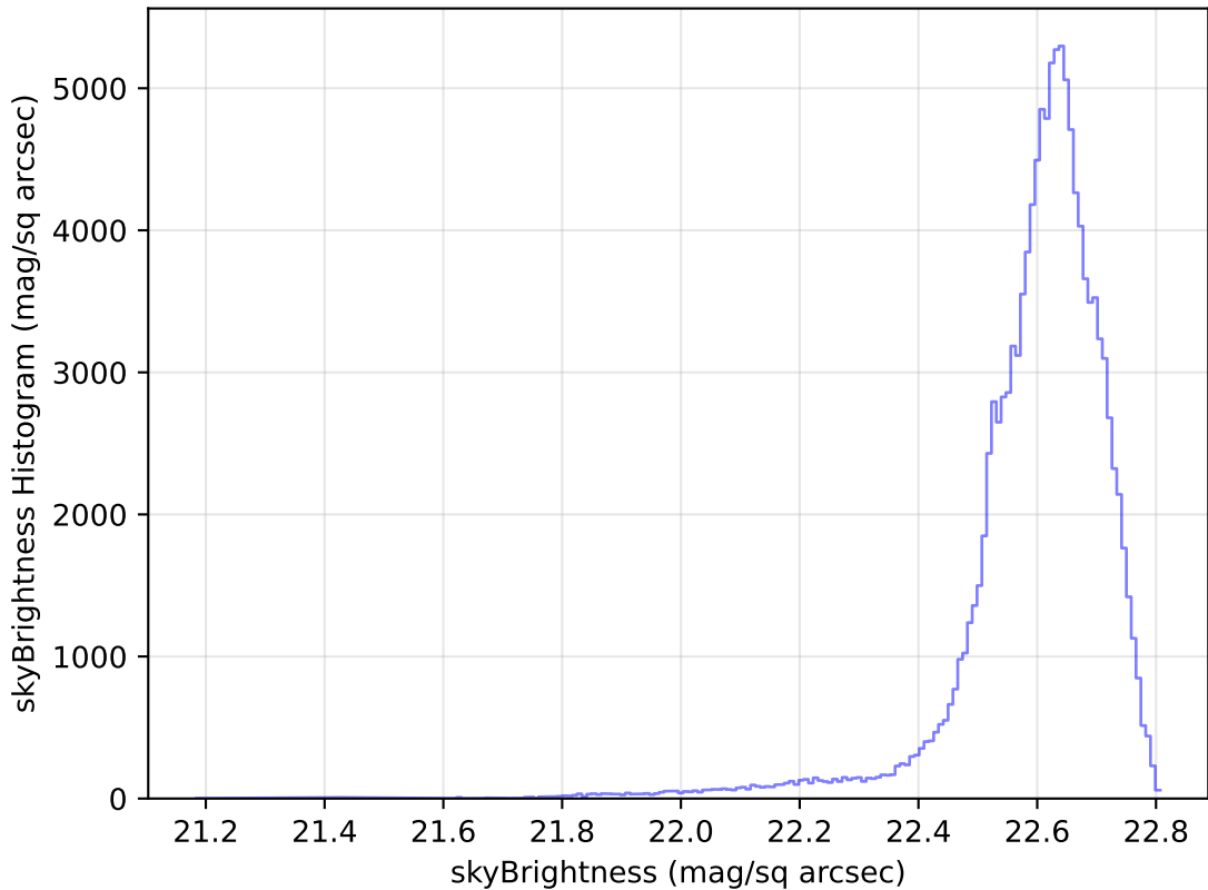
weather_cloudso35v3.4_10yrs WFD u band: skyBrightness Histogram
