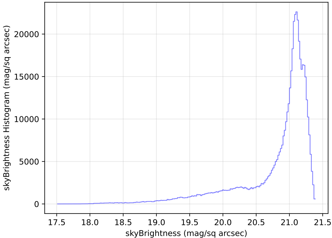
weather_cloudso35v3.4_10yrs WFD r band: skyBrightness Histogram
