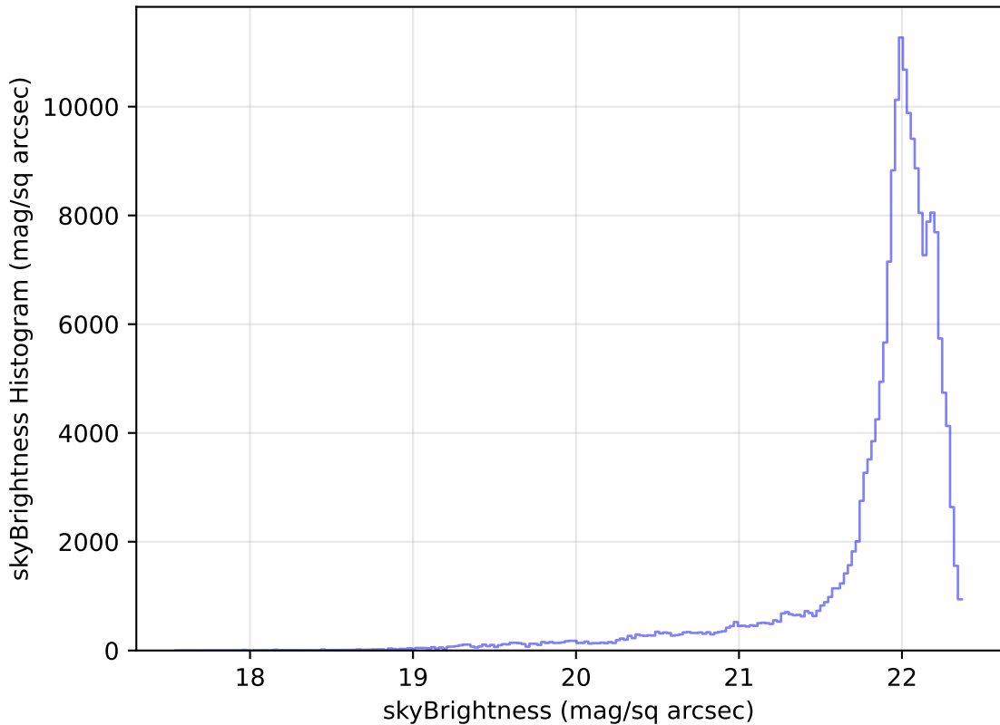
weather_cloudso35v3.4_10yrs WFD g band: skyBrightness Histogram
