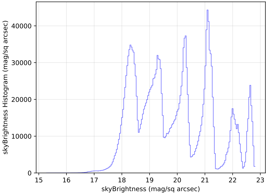
weather_cloudso35v3.4_10yrs WFD all bands: skyBrightness Histogram
