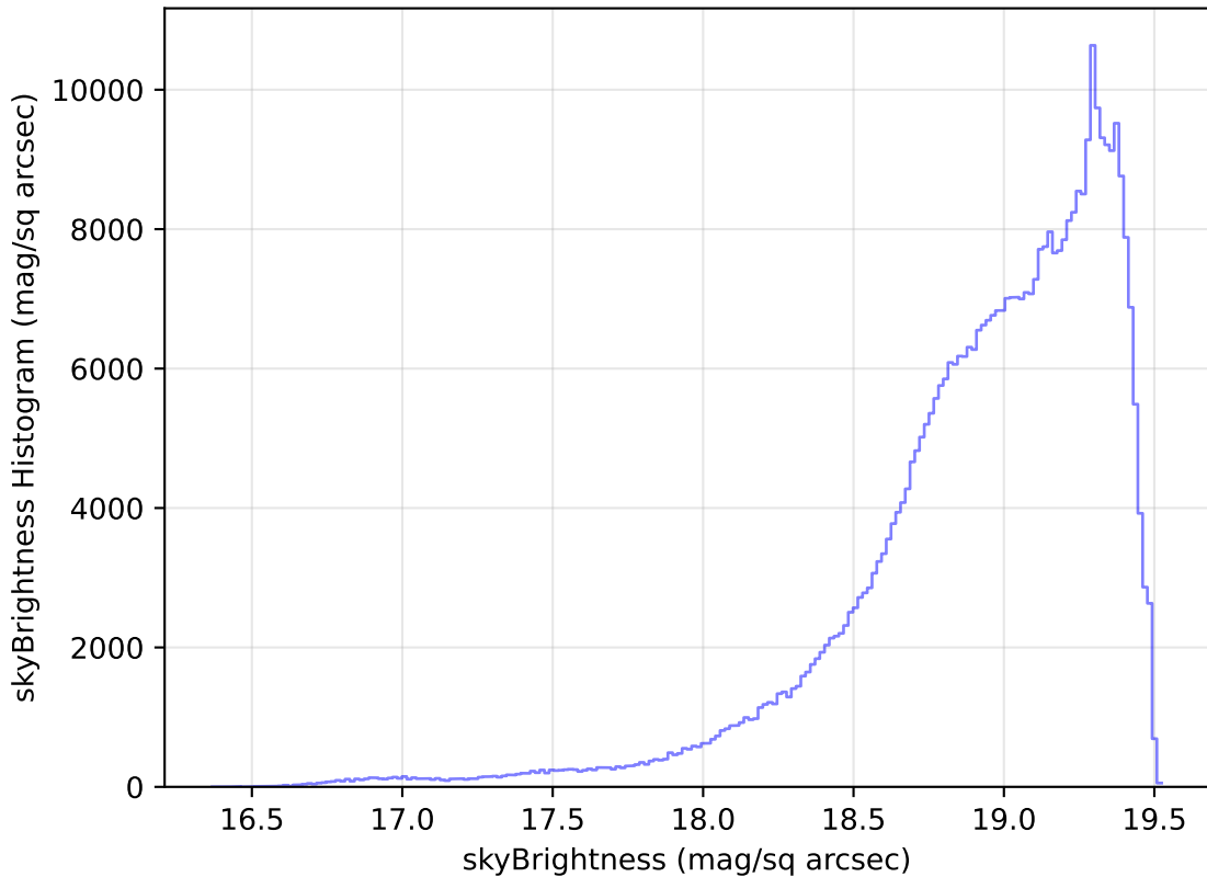
weather_cloudso35v3.4_10yrs All sky z band: skyBrightness Histogram
