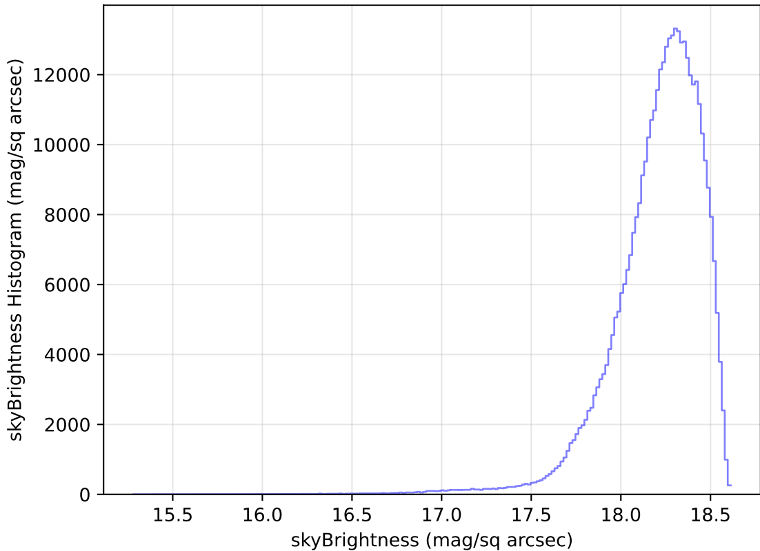
weather_cloudso35v3.4_10yrs All sky y band: skyBrightness Histogram
