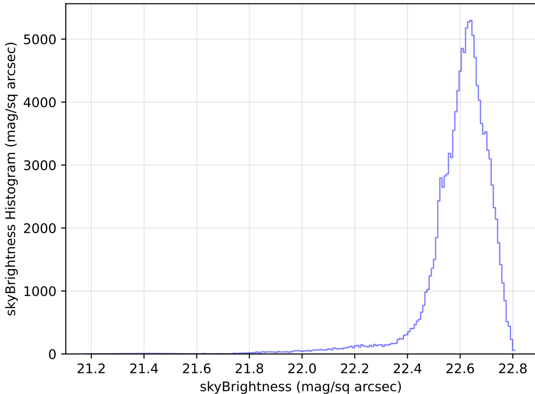
weather_cloudso35v3.4_10yrs All sky u band: skyBrightness Histogram
