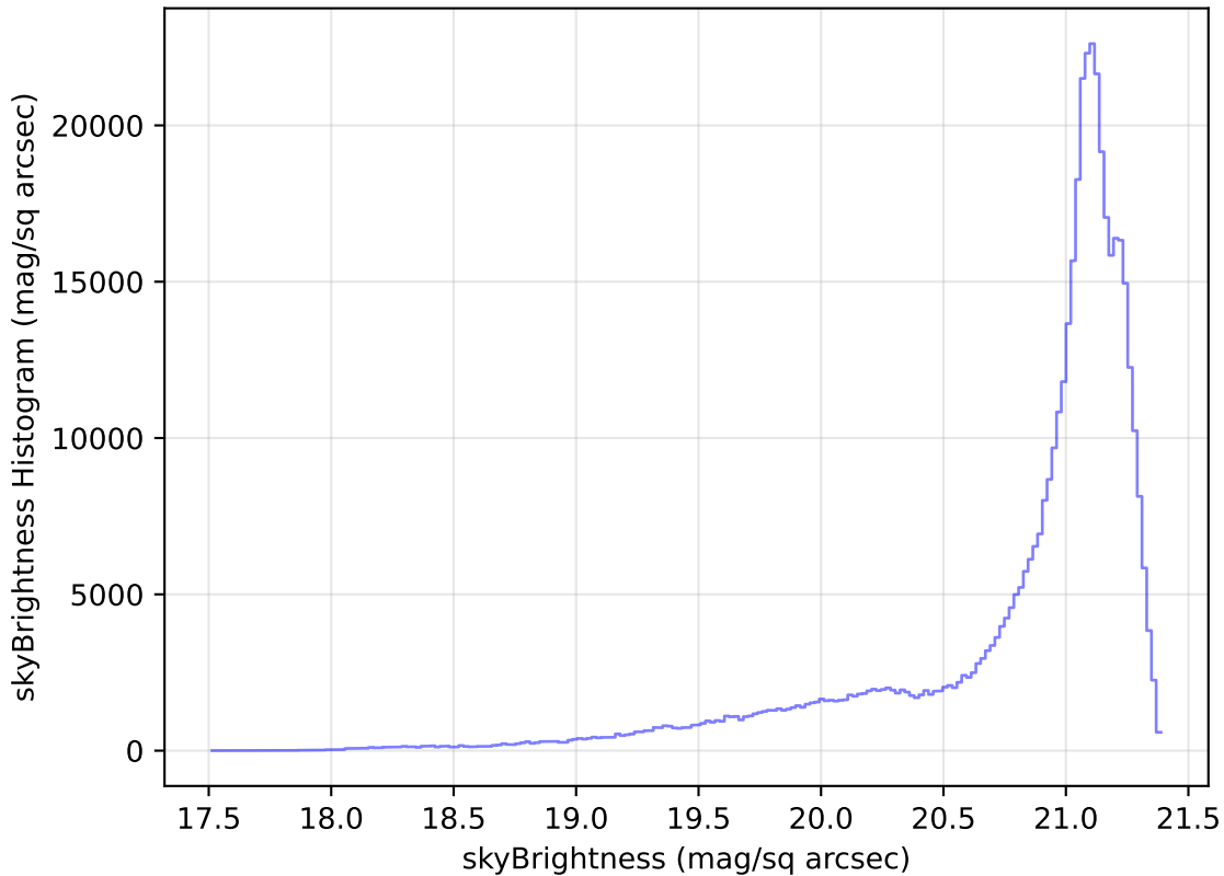
weather_cloudso35v3.4_10yrs All sky r band: skyBrightness Histogram
