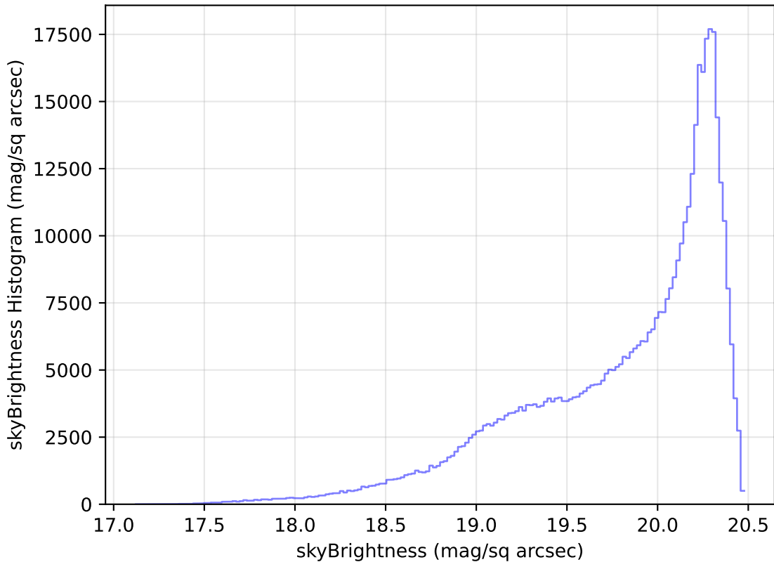
weather_cloudso35v3.4_10yrs All sky i band: skyBrightness Histogram
