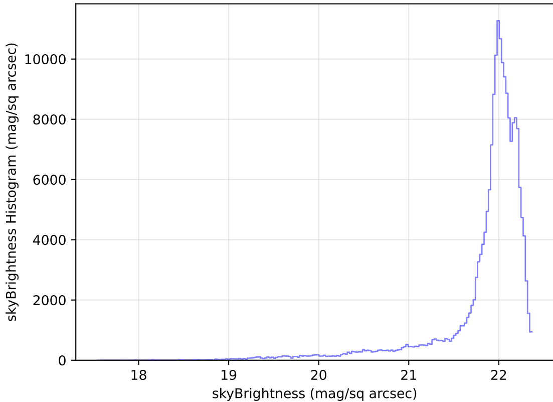
weather_cloudso35v3.4_10yrs All sky g band: skyBrightness Histogram
