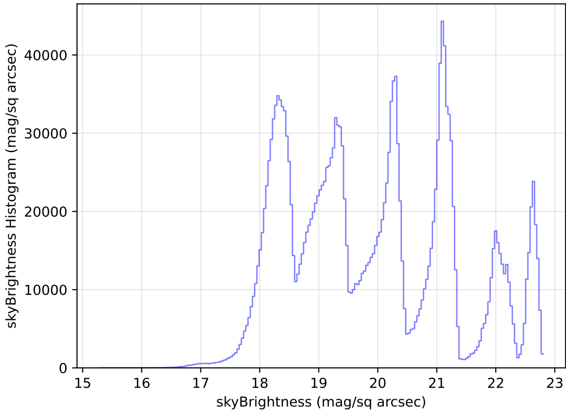
weather_cloudso35v3.4_10yrs All sky all bands: skyBrightness Histogram
