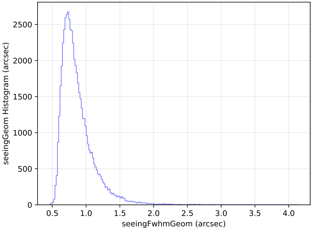
weather_cloudso35v3.4_10yrs Yr 1 i band: seeingGeom Histogram
