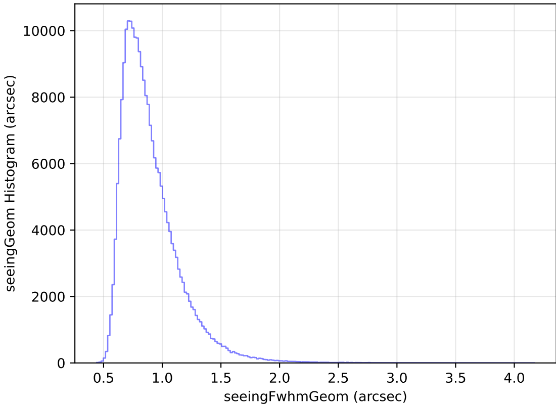
weather_cloudso35v3.4_10yrs Yr 1 all bands: seeingGeom Histogram
