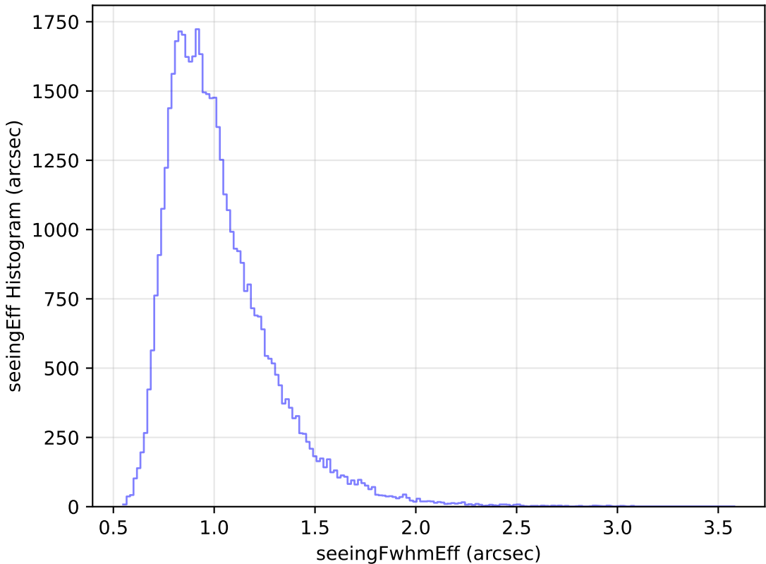
weather_cloudso35v3.4_10yrs Yr 1 y band: seeingEff Histogram
