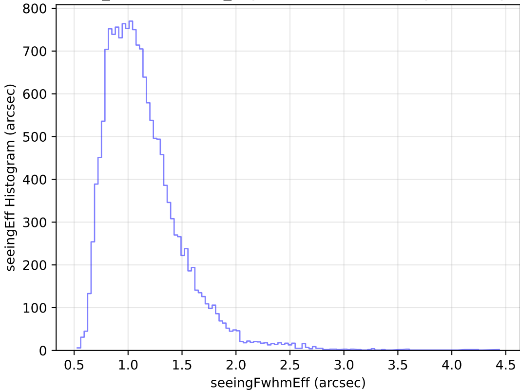
weather_cloudso35v3.4_10yrs Yr 1 u band: seeingEff Histogram
