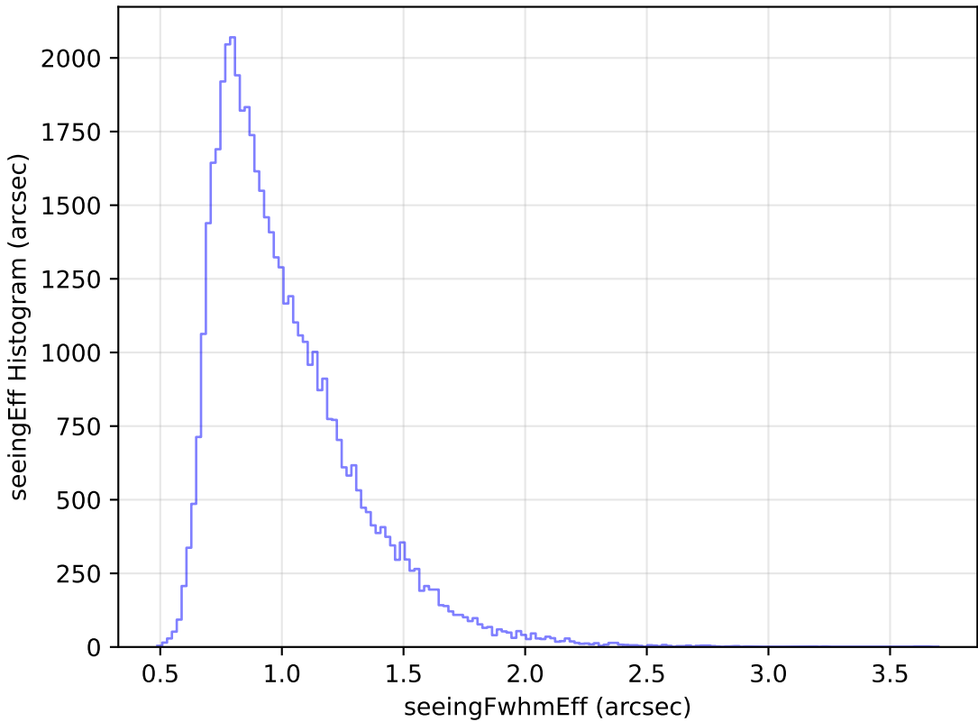
weather_cloudso35v3.4_10yrs Yr 1 r band: seeingEff Histogram
