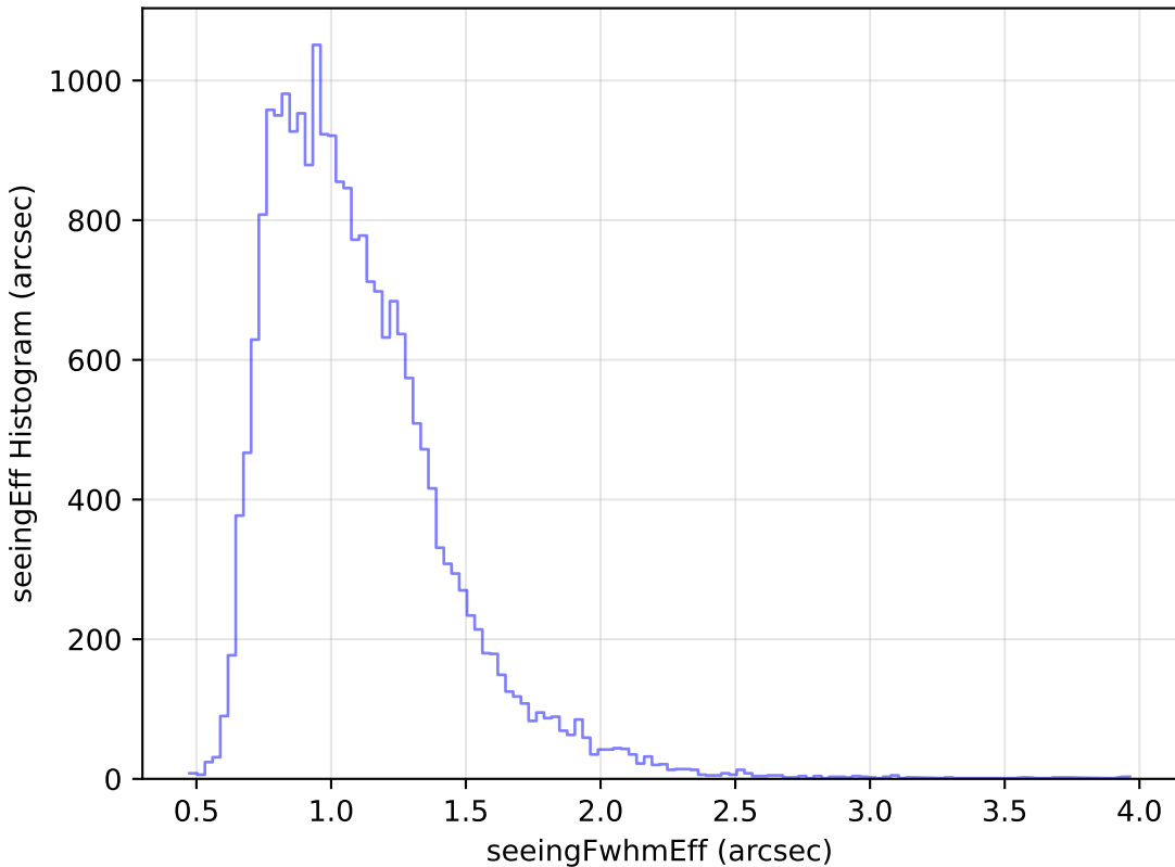
weather_cloudso35v3.4_10yrs Yr 1 g band: seeingEff Histogram
