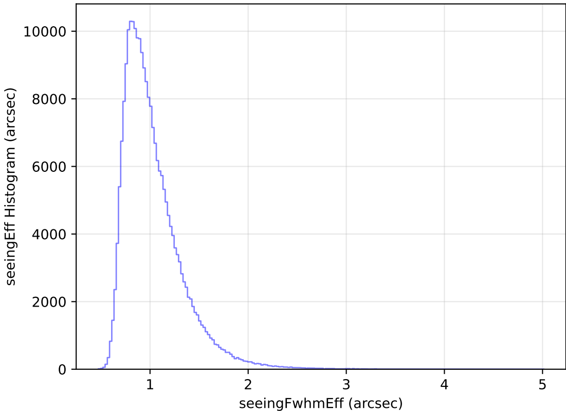
weather_cloudso35v3.4_10yrs Yr 1 all bands: seeingEff Histogram
