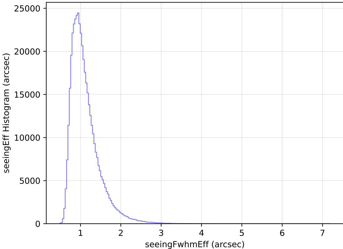
weather_cloudso35v3.4_10yrs WFD z band: seeingEff Histogram
