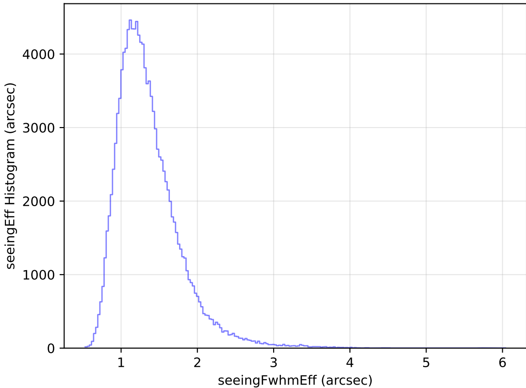
weather_cloudso35v3.4_10yrs WFD u band: seeingEff Histogram
