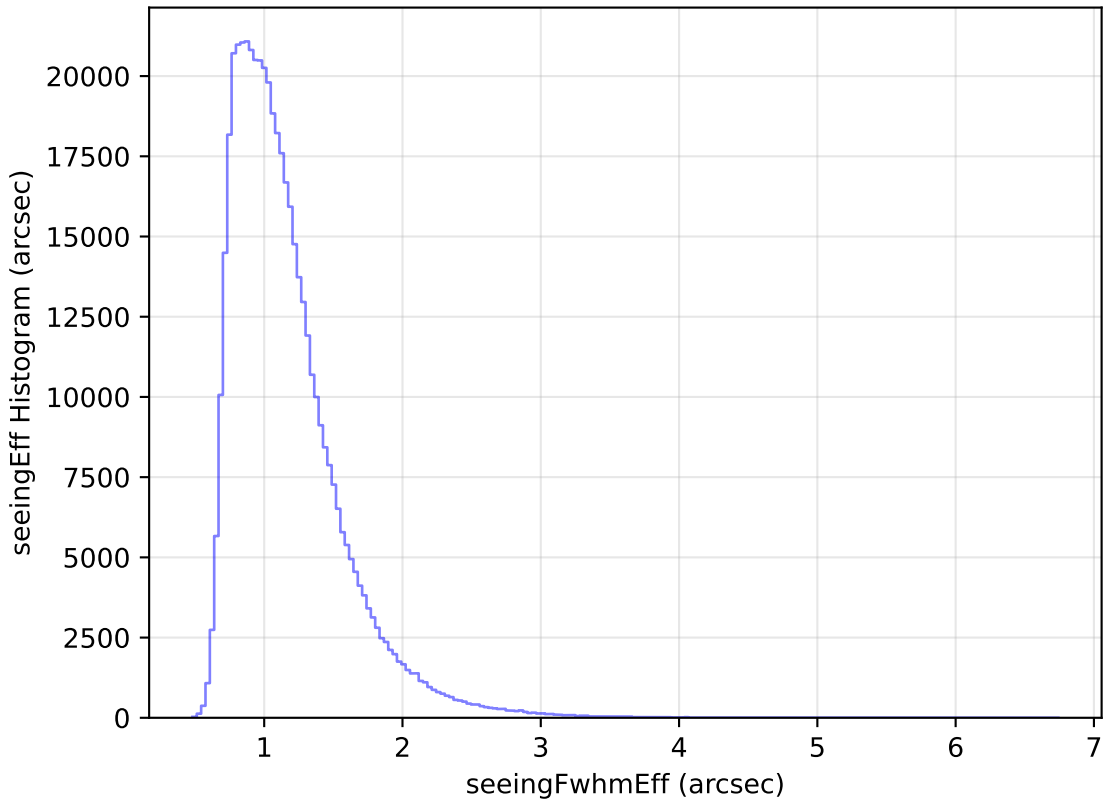
weather_cloudso35v3.4_10yrs WFD r band: seeingEff Histogram
