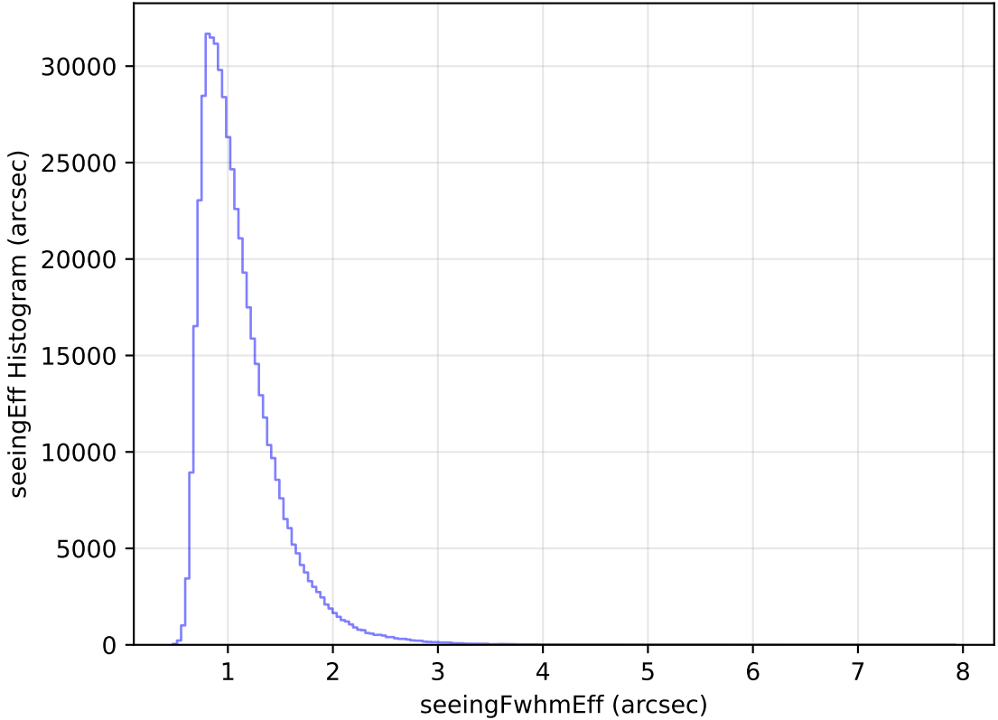
weather_cloudso35v3.4_10yrs WFD i band: seeingEff Histogram
