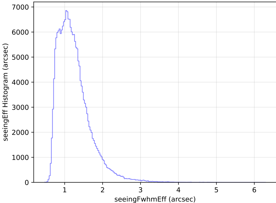
weather_cloudso35v3.4_10yrs WFD g band: seeingEff Histogram
