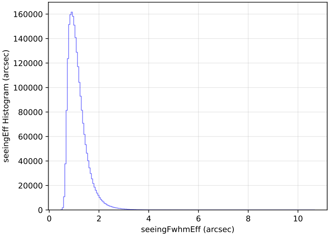
weather_cloudso35v3.4_10yrs WFD all bands: seeingEff Histogram
