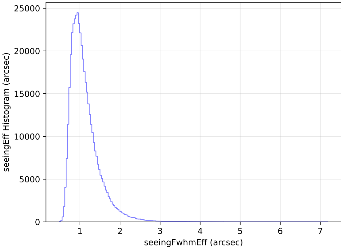
weather_cloudso35v3.4_10yrs All sky z band: seeingEff Histogram
