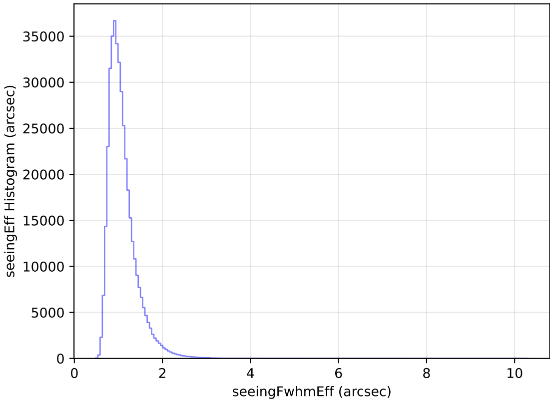
weather_cloudso35v3.4_10yrs All sky y band: seeingEff Histogram
