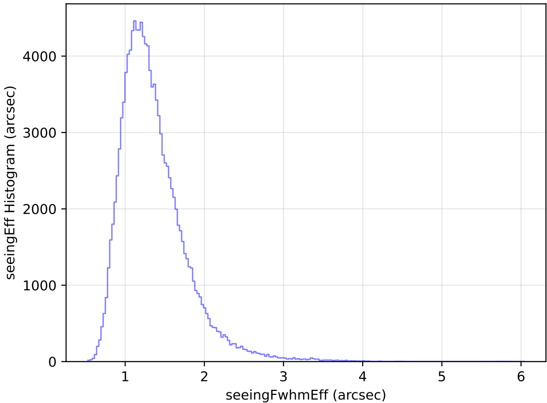
weather_cloudso35v3.4_10yrs All sky u band: seeingEff Histogram
