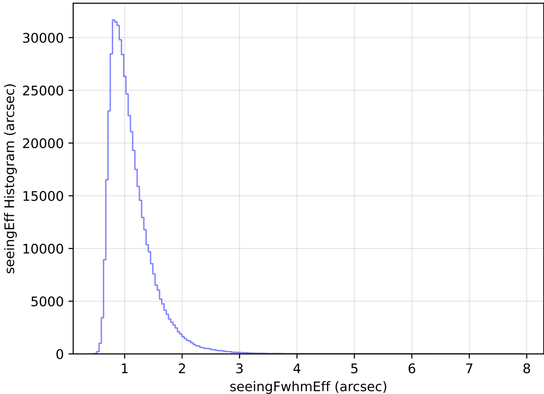
weather_cloudso35v3.4_10yrs All sky i band: seeingEff Histogram
