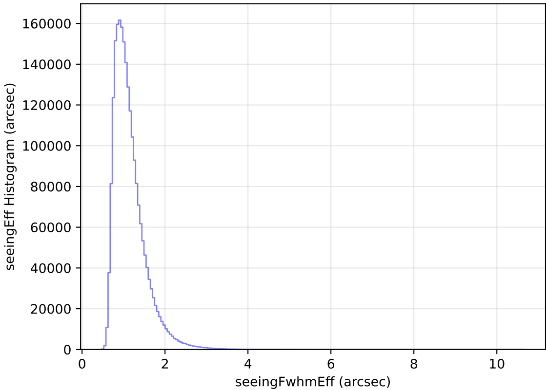
weather_cloudso35v3.4_10yrs All sky all bands: seeingEff Histogram
