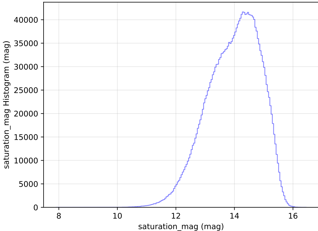
weather_cloudso35v3.4_10yrs WFD all bands: saturation_mag Histogram
