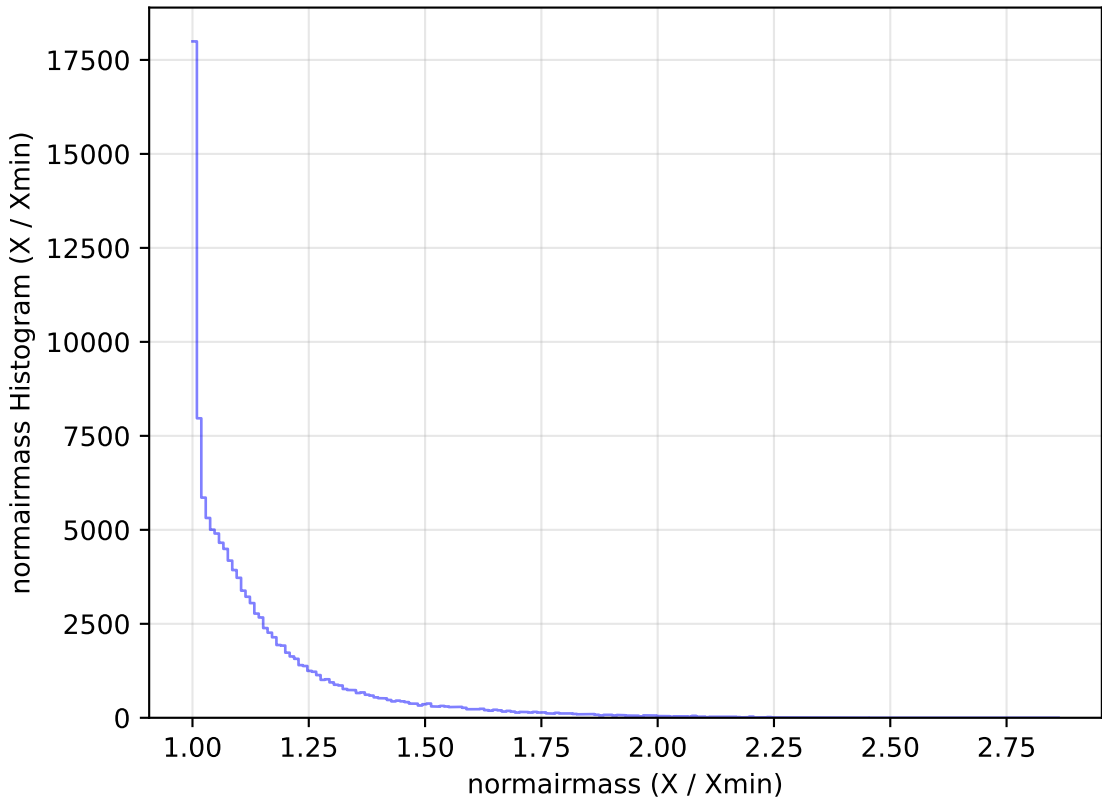
weather_cloudso35v3.4_10yrs WFD u band: normairmass Histogram
